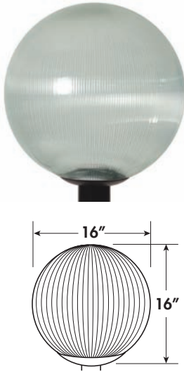
16" GLOBE POST
